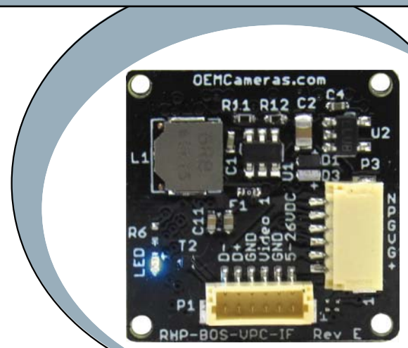
Low Profile Boson Accessory Module
